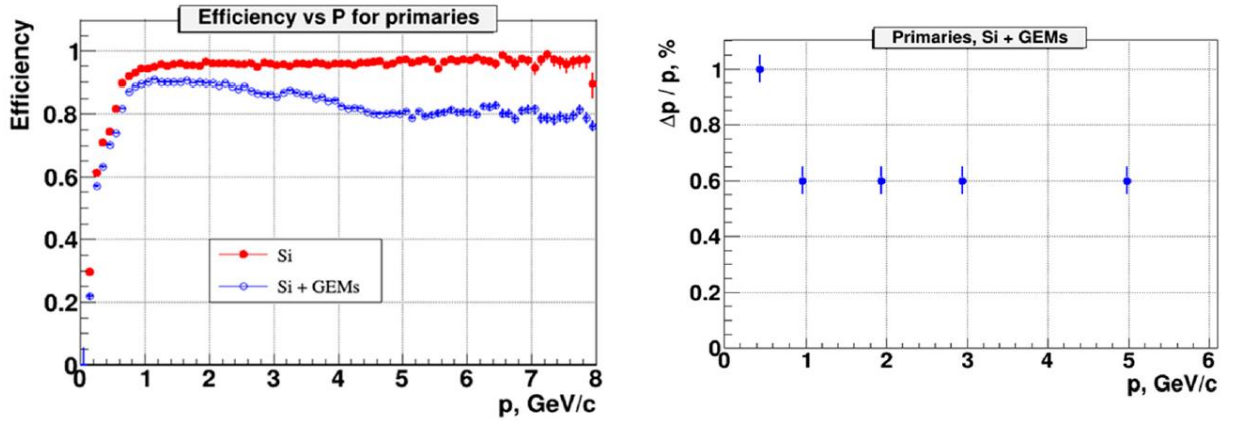
Fig.3.3.3.2 Left panel: Reconstruction efficiency as a function of 4 hits in the Si stations only (red histogram), and in the Si + GEM stations (blue histogram). Right panel: Momentum resolution for primary tracks emitted in the central Au + Au collisions at a beam kinetic energy of 4 A GeV reconstructed by the BM@N hybrid tracking system as a function of momentum.
