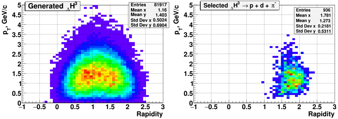
Figure 3.2.2.5 Left plot: distribution of \Lambda H^3 generated in Au+Au collisions at the beam kinetic energy of 4 AGeV in the phase space of the \Lambda H^3 transverse momentum and rapidity in the laboratory frame. Right plot: distribution of reconstructed \Lambda H^3 as a function of the \Lambda H^3 transverse momentum and rapidity.
