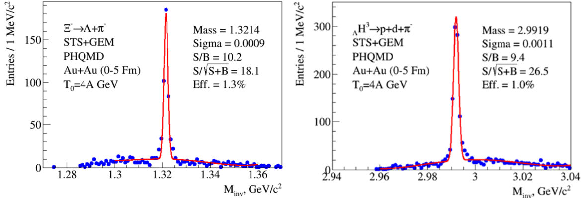
Figure 3.2.2.4 Left plot: Signal of \Xi^- hyperon in the invariant mass spectrum of simulated ( \Lambda , \pi^- ) reconstructed in the hybrid STS+GEM tracker. Right plot: Signal of \Lambda H^3 in the invariant mass spectrum of simulated ( p , d , \pi^- ) reconstructed in the hybrid STS+GEM tracker.
