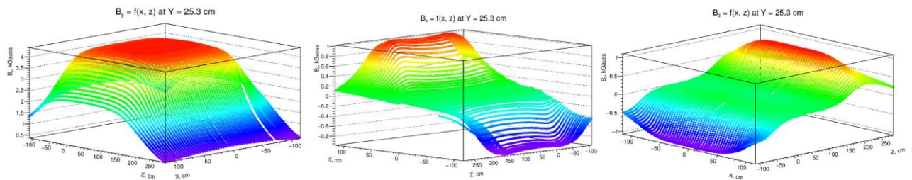
Figure 3.10.9. Two dimensional (X-Z) distributions of the magnetic field components B_y , B_x , B_z (kGauss) measured in the horizontal plane at Y=25 cm from the magnet median plane.
